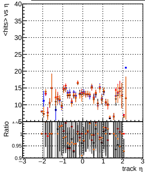
mean hit DQM_testMkFitFit_initialStepReso DQM_testMkFitFit_initialStepReso DQM_testMkFitFit_initialStepReso_wRejection100
