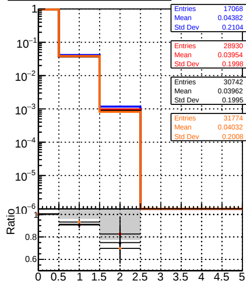
mean hit — DQM_testMkFit_initialStepReso — DQM_testMkFitFit_initialStepReso — DQM_testMkFitFit_initialStepReso_wRejection100
