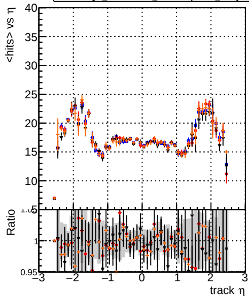
mean hit DQM_original4 DQM_testMkFitFit_initialStepReso DQM_testMkFitFit_initialStepReso DQM_testMkFitFit_initialStepReso_wRejection100
