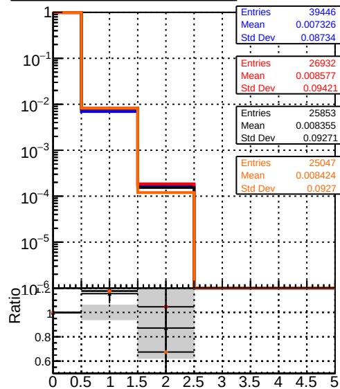
mean hit DQM_original4 DQM_testMkFit_initialStepReso DQM_testMkFitFit_initialStepReso DQM_testMkFitFit_initialStepReso_wRejection100
