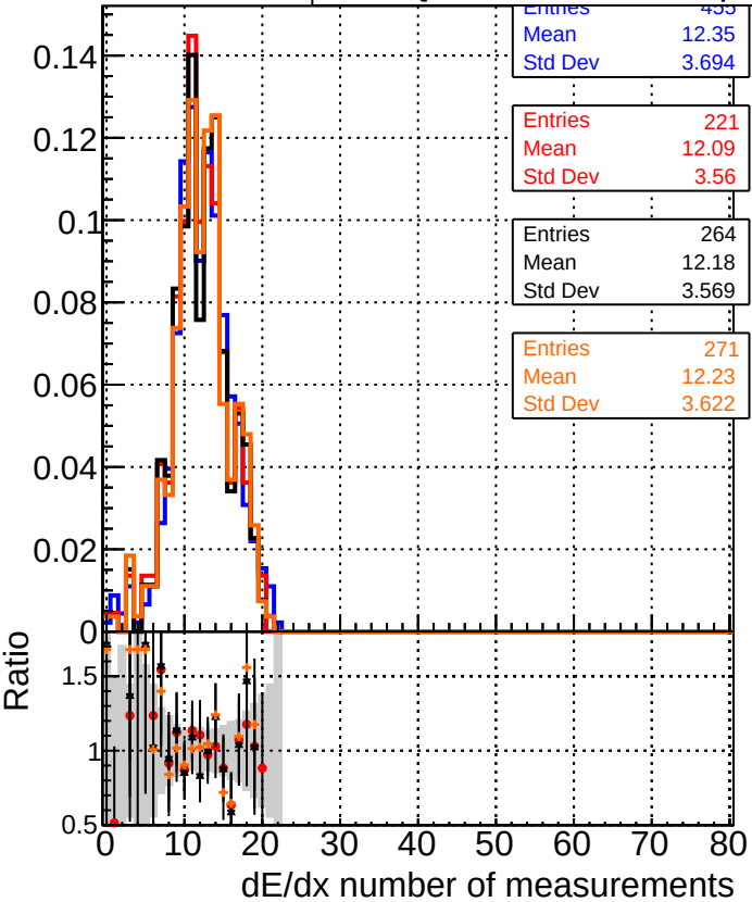
— DQM_original4 — DQM_testMkFit_initialStepReso — DQM_testMkFitFit_initialStepReso — DQM_testMkFitFit_initialStepReso_wRejection100
