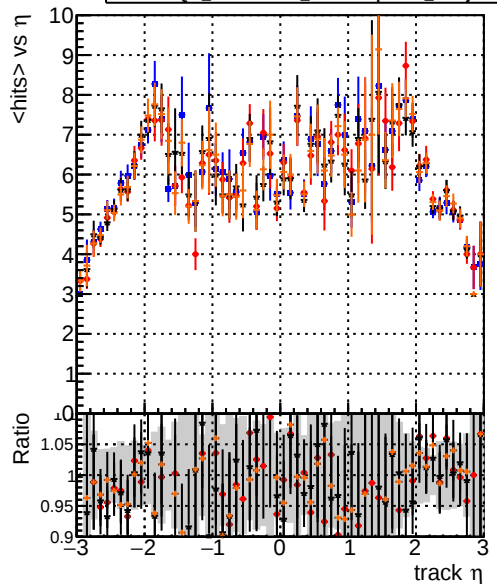
DQM_testMkFit_initialStepReso DQM_testMkFitFit_initialStepReso DQM_testMkFitFit_initialStepReso_wRejection100 mean hit
