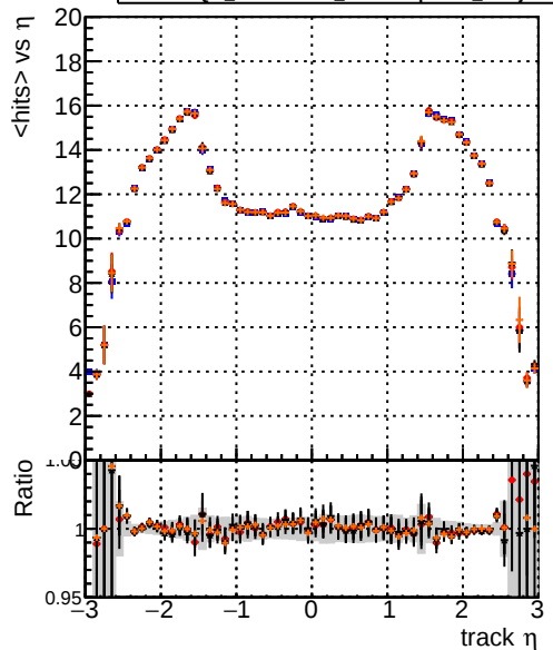
Legend for mean hits vs \eta : Blue line: DQM_original4 Red line: DQM_testMkFit_initialStepReso Black line: DQM_testMkFitFit_initialStepReso Orange line: DQM_testMkFitFit_initialStepReso_wRejection100 mean hits
