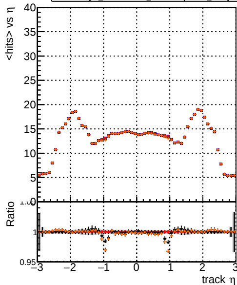
mean hit DQM_original4 DQM_testMkFit_initialStepReso DQM_testMkFitFit_initialStepReso DQM_testMkFitFit_initialStepReso_wRejection100
