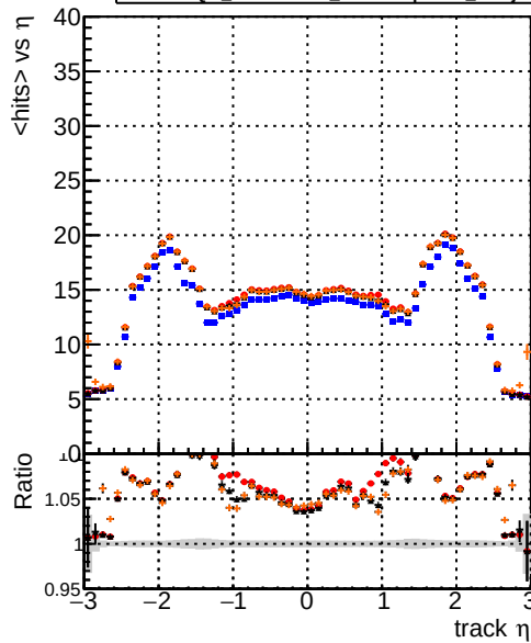
mean hit DQM_original14 DQM_testMkFit_initialStepReso DQM_testMkFitFit_initialStepReso DQM_testMkFitFit_initialStepReso_wRejection100
