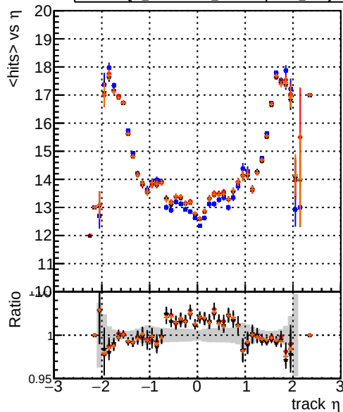
mean hits vs \eta Legend: Blue line: DQM_testMkFit_initialStepReso Red line: DQM_testMkFitFit_initialStepReso Black line: DQM_testMkFitFit_initialStepReso Orange line: DQM_testMkFitFit_initialStepReso_wRejection100
