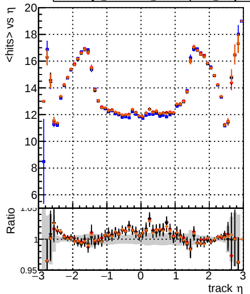
Legend: DQM_original4, DQM_testMkFit_initialStepReso, DQM_testMkFitFit_initialStepReso, DQM_testMkFitFit_initialStepReso_wRejection100 mean hits
