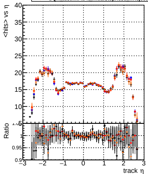
mean hits vs \eta DQM_original4 DQM_testMkFit_initialStepReso DQM_testMkFitFit_initialStepReso DQM_testMkFitFit_initialStepReso_wRejection100
