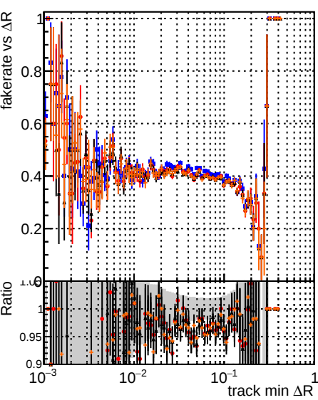
Fake rate vs \Delta R(\text{track, jet}) DOM original DOM fit DOM fit initialStepReso DOM fit initialStepReso wRejection100
