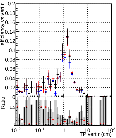
Efficiency vs vertpos DQM_original4 DQM_testMkFit_initialStepReso DQM_testMkFitFit_initialStepReso
