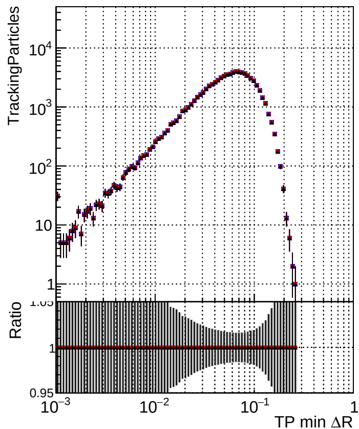
N of simulated tracks vs \Delta R (TP, jet) DQM_original4 DQM_testMkFit_initialStepReso DQM_testMkFitFit_initialStepReso
