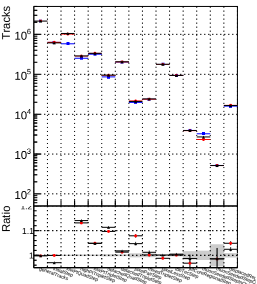
Number DQM_original4 DQM_testMkFit_initialStepReso DQM_testMkFitFit_initialStepReso
