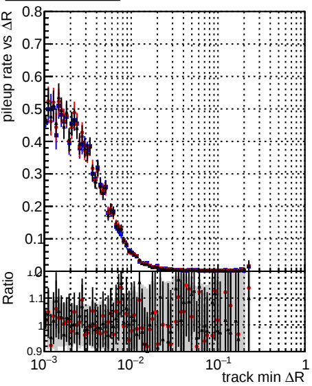
Legend: - \Delta R original - \Delta R testMkFit_initialStepReso - \Delta R testMkFitFit_initialStepReso
