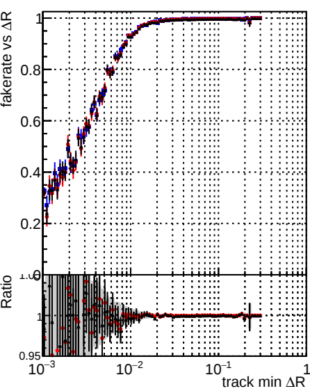
Legend: - \Delta R original - \Delta R testMkFit_initialStepReso - \Delta R testMkFitFit_initialStepReso
