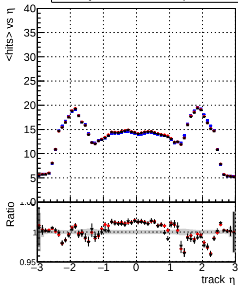
DQM_original4 DQM_testMkFit_initialStepReso DQM_testMkFitFit_initialStepReso mean hit
