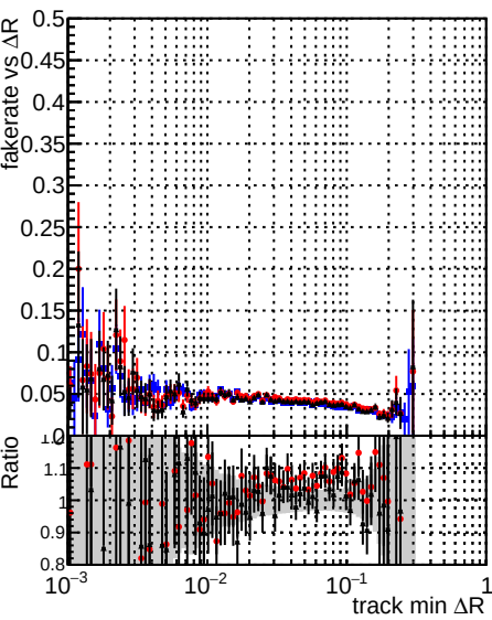
Fake rate vs \Delta R(\text{track}, \text{jet}) Legend: DQM_original4 DQM_testMkFit_initialStepReso DQM_testMkFitFit_initialStepReso
