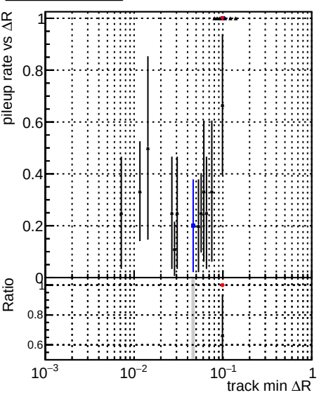
Legend: DQM_original (blue), DQM_testMkFit_initialStepReso (red), DQM_testMkFitFit_initialStepReso (black)
