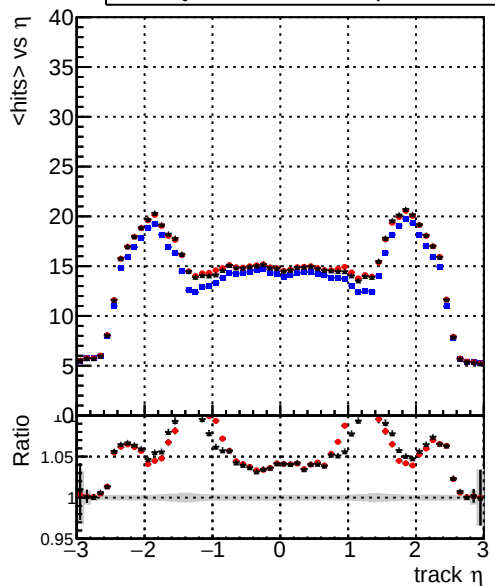
mean hits vs \eta — DQM_original4 — DQM_testMkFit_initialStepReso — DQM_testMkFitFit_initialStepReso
