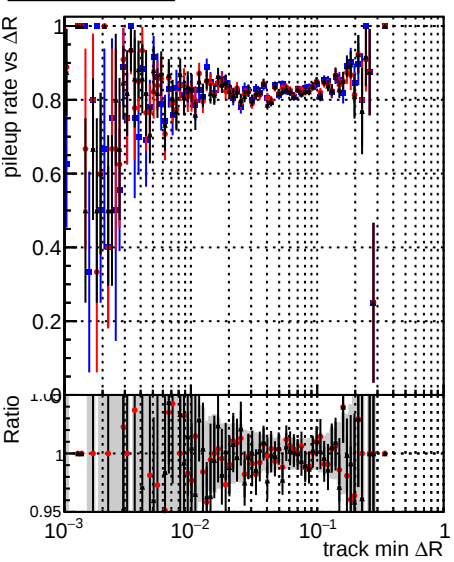
—•— DQM_original4 —•— DQM_testMkFit_initialStepReso —•— DQM_testMkFitFit_initialStepReso
