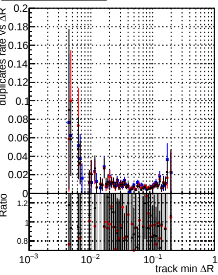
—•— DQM_original4 —•— DQM_testMkFit_initialStepReso —•— DQM_testMkFitFit_initialStepReso
