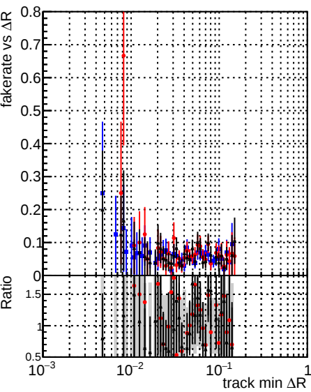
Legend: DQM_original (blue squares), DQM_testMkFit_initialStepReso (red circles), DQM_testMkFitFit_initialStepReso (black triangles)
