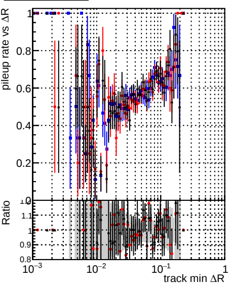
Legend: DQM_original (blue squares), DQM_testMkFit_initialStepReso (red circles), DQM_testMkFitFit_initialStepReso (black triangles)
