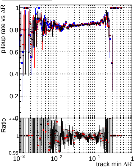
Legend: DQM original (blue line with dots), DQM testMkFit_initialStepReso (red line with dots), DQM testMkFitFit_initialStepReso (black line with dots)
