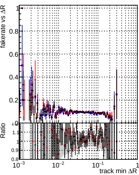
Legend: DQM original (blue line with dots), DQM testMkFit_initialStepReso (red line with dots), DQM testMkFitFit_initialStepReso (black line with dots)
