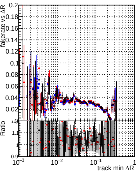
Legend: \bullet DQM_original4 \bullet DQM_testMkFit_initialStepReso \bullet DQM_testMkFitFit_initialStepReso
