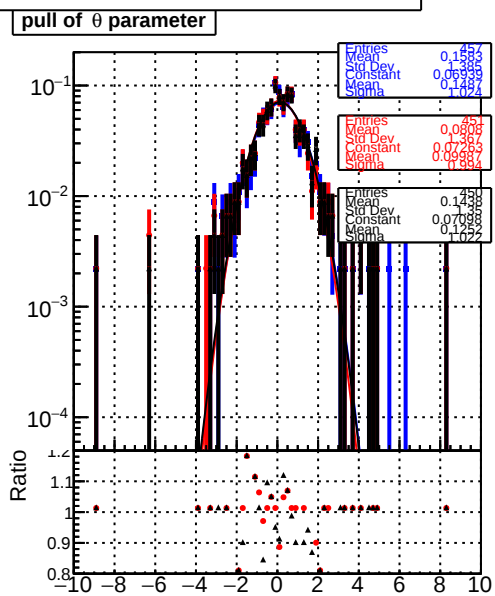
Legend: BDM (black), BDM + initialStepReso (blue), BDM + initialStepReso + BDM testMRFit (red)
