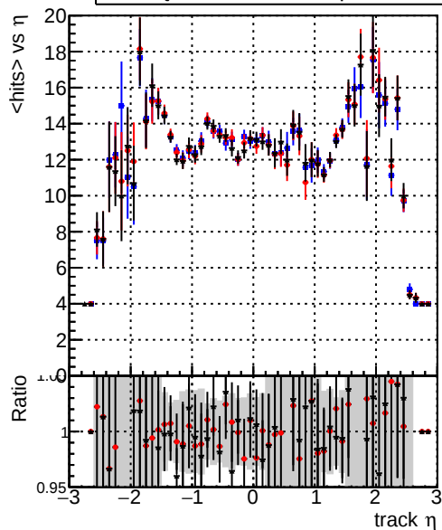
mean hits — DQM_original4 — DQM_testMkFit_initialStepReso — DQM_testMkFitFit_initialStepReso
