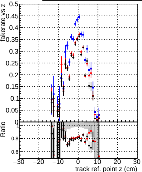
Fake rate vs verpos DQM_original DQM_testMkFit_initialStepReso DQM_testMkFitFit_initialStepReso
