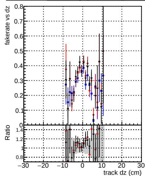
Fake rate vs dz DOM original4 DOM testMKFit initialStepReso DOM testMKFit initialStepReso
