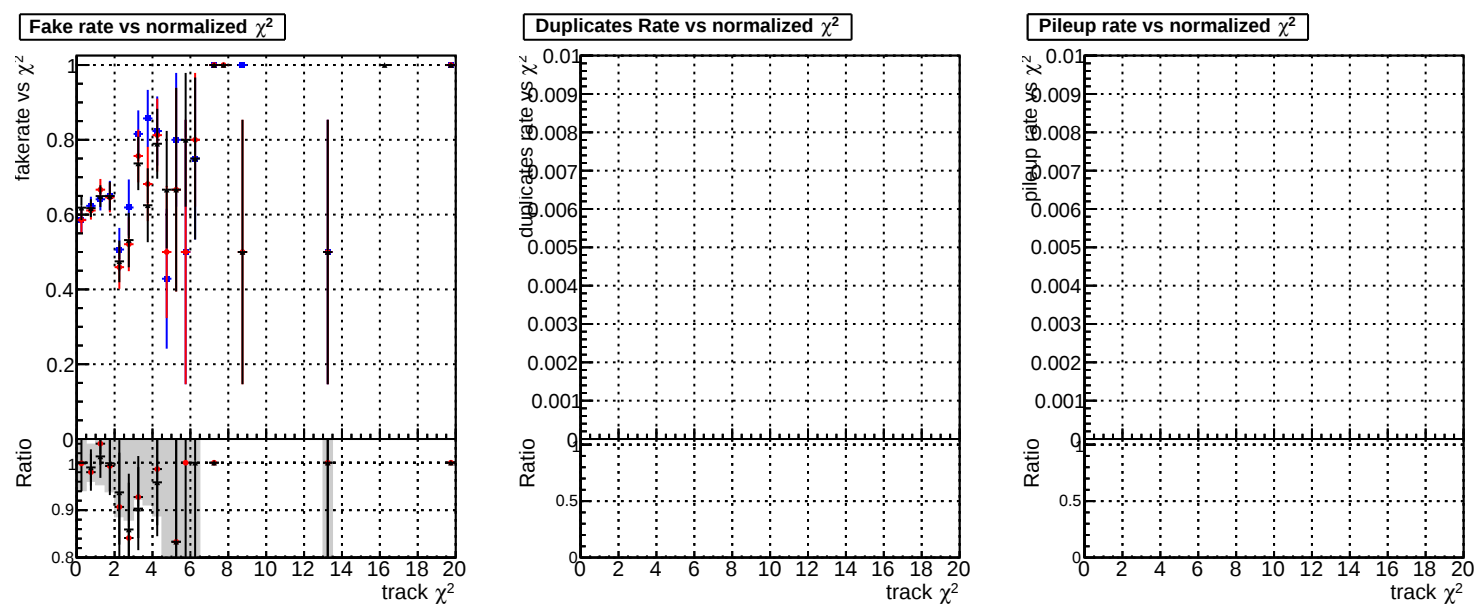
Fake rate vs. DOM original4 DOM testMKFit initialStepReso DOM testMKFit initialStepReso
