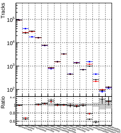
Number Legend: DQM_original4 DQM_testMkFit_initialStepReso DQM_testMkFitFit_initialStepReso
