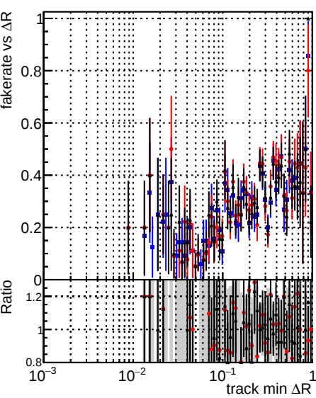
Legend: DQM_original4 (blue), DQM_testMkFit_initialStepReso (red), DQM_testMkFitFit_initialStepReso (black)
