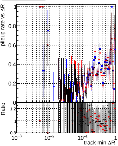
Legend: DQM_original4 (blue), DQM_testMkFit_initialStepReso (red), DQM_testMkFitFit_initialStepReso (black)
