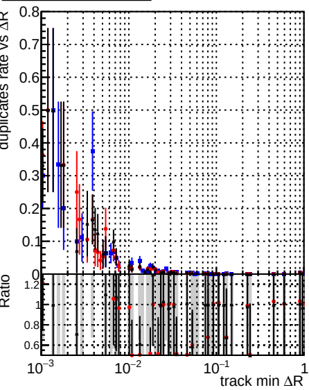
Legend: DQM_original (blue squares), DQM_testMkFit_initialStepReso (red circles), DQM_testMkFitFit_initialStepReso (black crosses)
