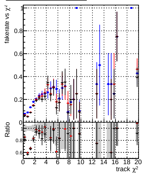
Fake rate vs. DOM original4 DOM testMKFit initialStepReso DOM testMKFit initialStepReso
