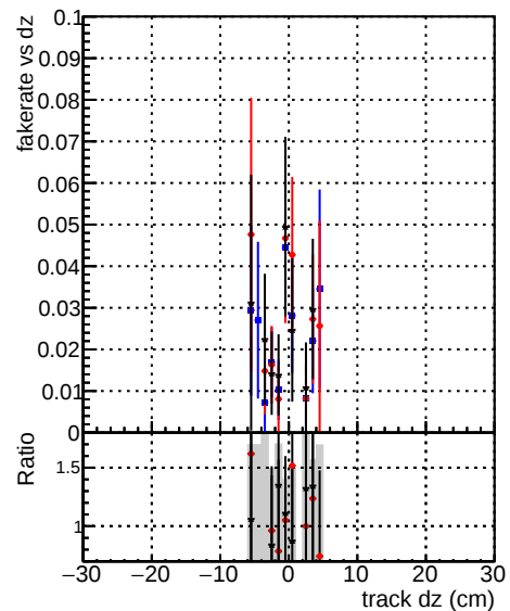
Fake rate vs dz Legend: DOM original4 DOM testMKFit initialStepReso DOM testMKFit initialStepReso
