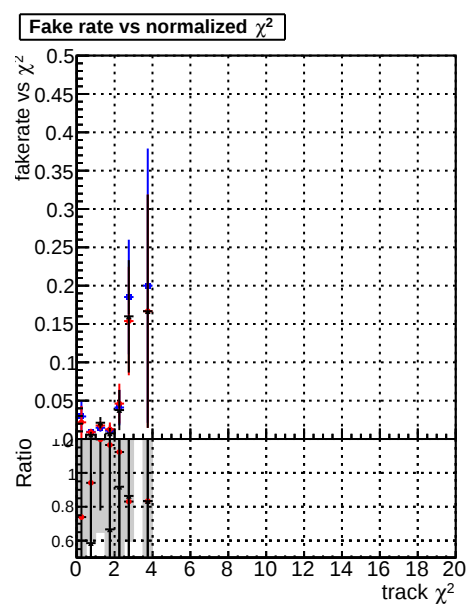
Fake rate vs. DOM original4 DOM testMKFit DOM testMKFit initialStepReso
