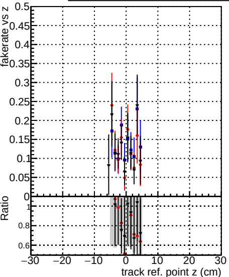
Fake rate vs verpos —●— DQM_original4 —●— DQM_testMkFit_initialStepReso —●— DQM_testMkFitFit_initialStepReso
