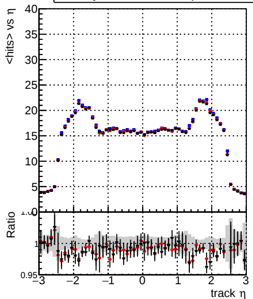
mean hits vs \eta Legend: DQM_original4 (blue line), DQM_testMkFit_initialStepReso (red line), DQM_testMkFitFit_initialStepReso (black line)
