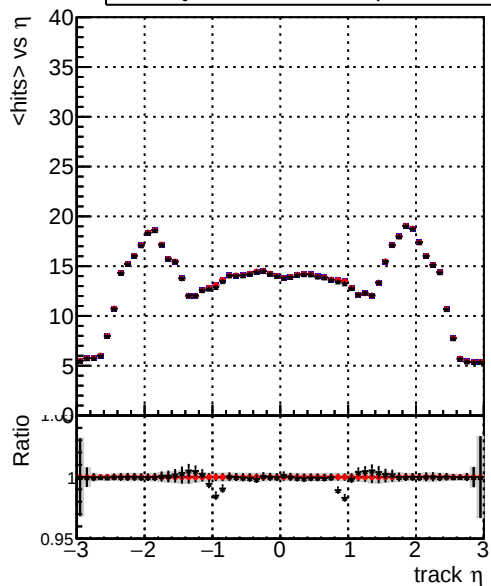
mean hits DQM_original4 DQM_testMkFit_initialStepReso DQM_testMkFitFit_initialStepReso
