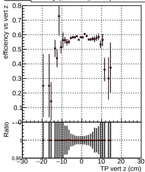
Efficiency vs vert z —●— DQM_original4 —●— DQM_testMkFit_initialStepReso —●— DQM_testMkFitFit_initialStepReso
