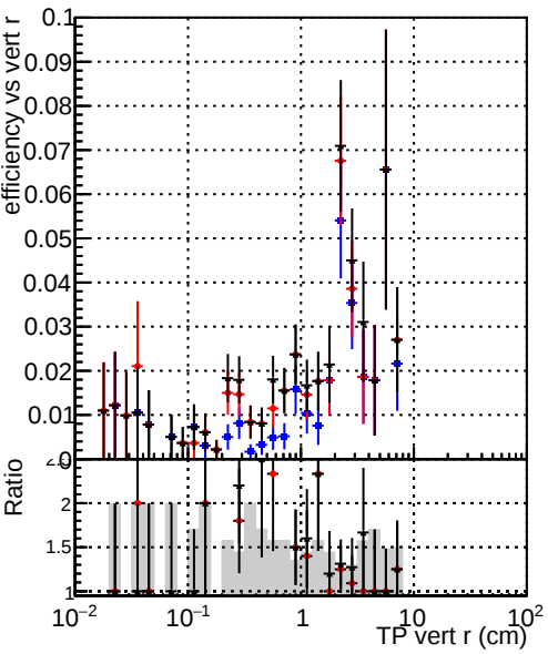
Efficiency vs TP vert r (cm) Legend: DQM_original4 DQM_testMkFit_initialStepReso DQM_testMkFitFit_initialStepReso
