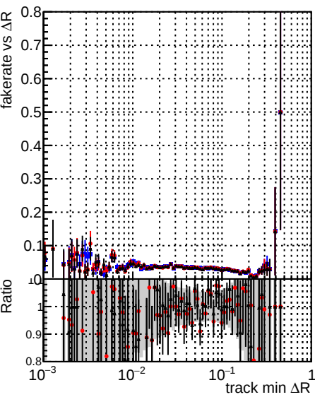
Legend: \square DQM_original4 \square DQM_testMkFit_initialStepReso \square DQM_testMkFitFit_initialStepReso
