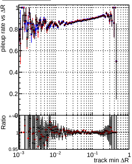
Legend: \square DQM_original4 \square DQM_testMkFit_initialStepReso \square DQM_testMkFitFit_initialStepReso
