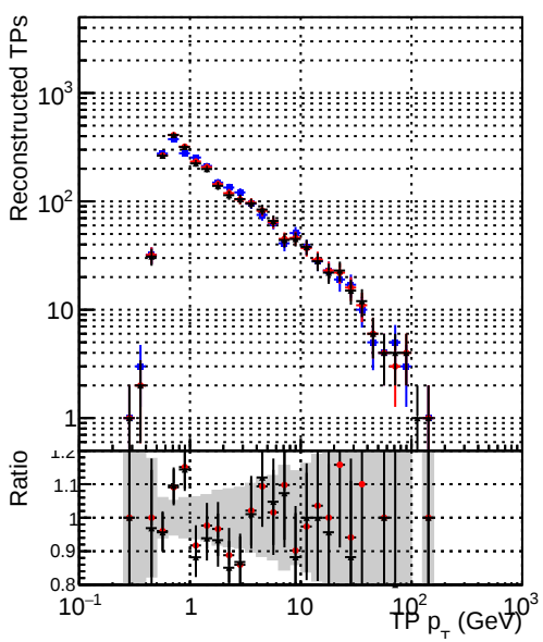
Legend: DQM_original4 (blue circle), DQM_testMkFit_initialStepReso (red circle), DQM_testMkFitFit_initialStepReso (black cross)
