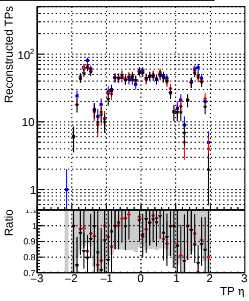
Legend: DQM_original4 (blue circle), DQM_testMkFit_initialStepReso (red circle), DQM_testMkFitFit_initialStepReso (black cross)
