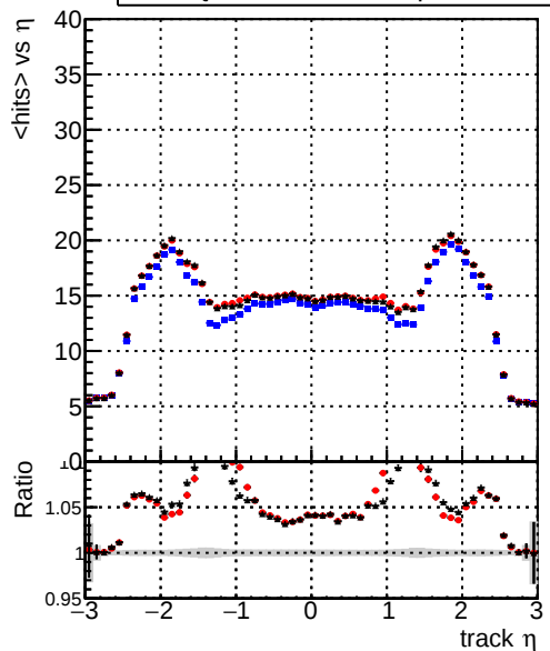
mean hits — DQM_original4 — DQM_testMkFit_initialStepReso — DQM_testMkFitFit_initialStepReso
