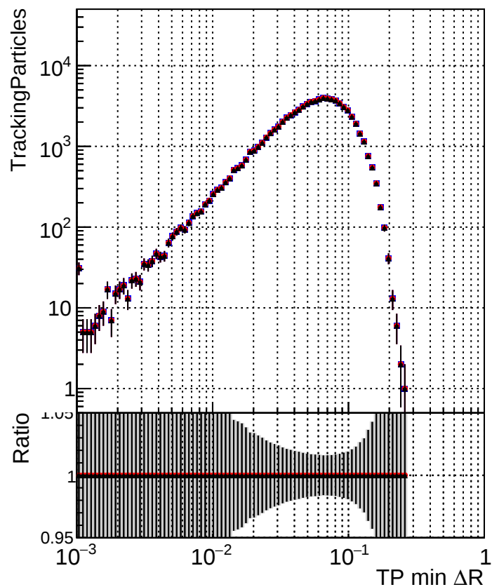
N of simulated tracks vs TP \Delta R (TP, jet) DQM_original3 DQM_testMk_initialStepReso DQM_testMkFitExportFit_initialStepReso
