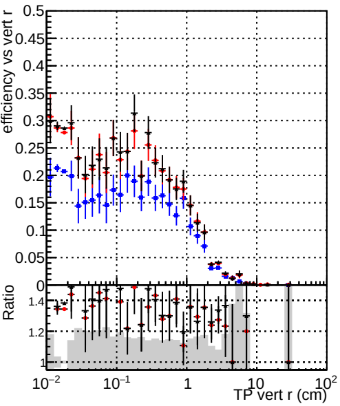
Efficiency vs vertpos Legend: DQM_original3 DQM_testMk_initialStepReso DQM_testMkFitExportFit_initialStepReso
