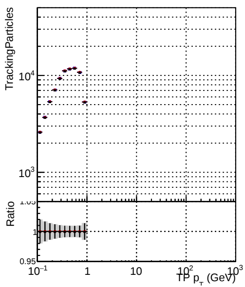
● DQM_original3 ● DQM_testMk_initialStepReso ● DQM_testMkFitExportFit_initialStepReso
