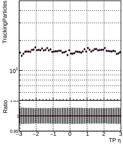
● DQM_original3 ● DQM_testMk_initialStepReso ● DQM_testMkFitExportFit_initialStepReso
