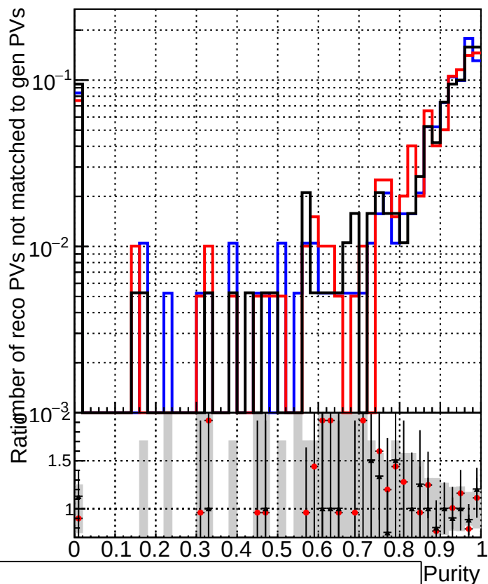
RecoPVAssoc2GenPVNotMatched_Purity
