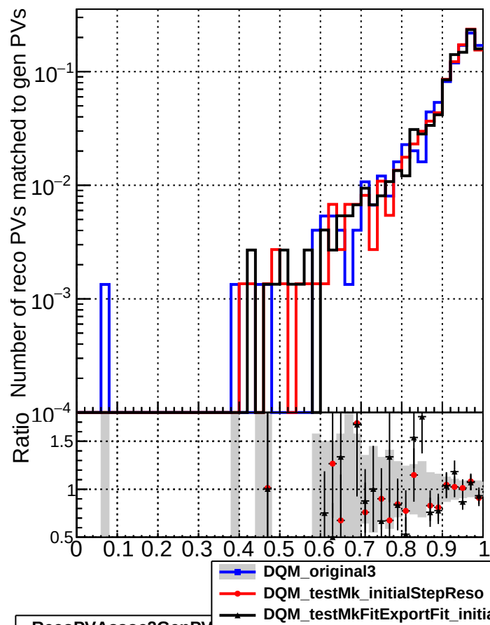
RecoPVAssoc2GenPVmatched_missing
