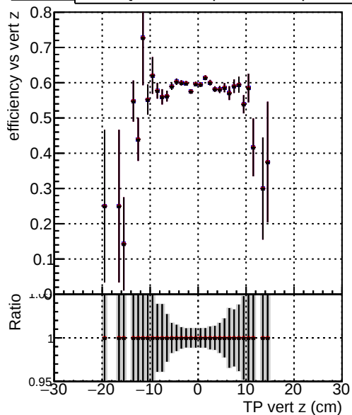
Efficiency vs. TP vert z —•— DQM_original3 —•— DQM_testMk_initialStepReso —•— DQM_testMkFitExportFit_initialStepReso
