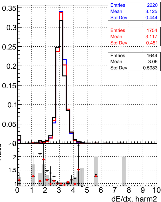
—■ DQM_original3 —● DQM_testMk_initialStepReso —▲ DQM_testMkFitExportFit_initialStepReso
